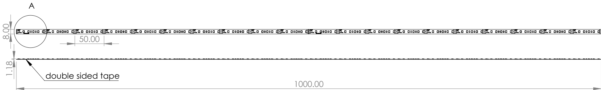
DETAIL A
